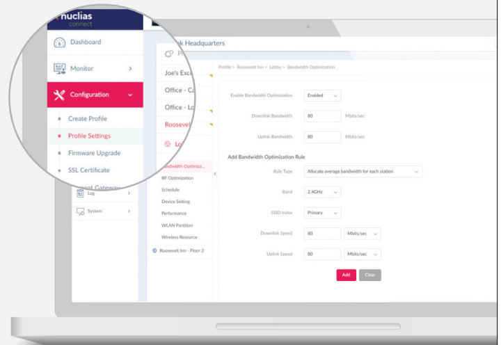
▲ Network-Wide Configuration
